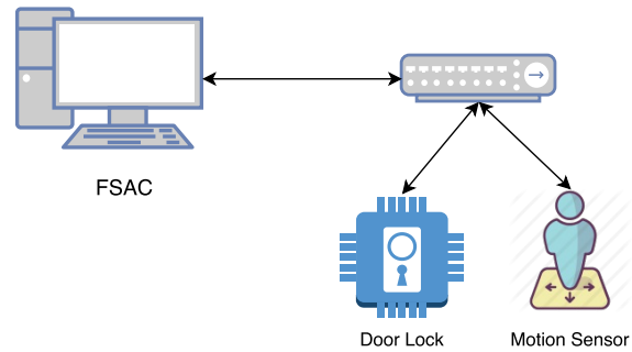
Figure 3: FSAC to controller
